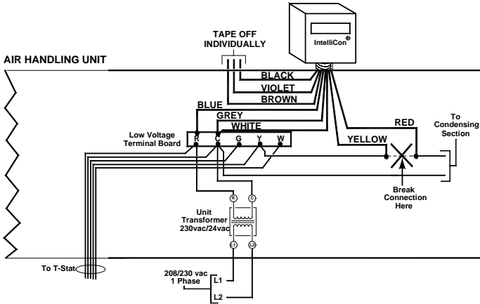
24 Vac Power / Control
