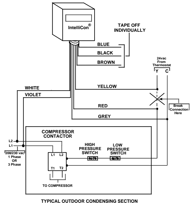
Typical Split Unit Condenser Section
