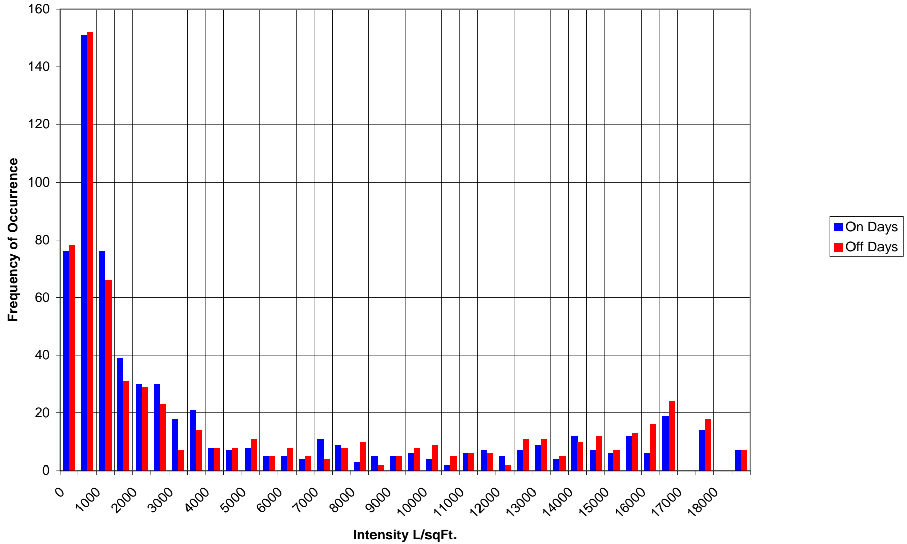
Atlantic City - County Office Building Solar Influence Histogram (12/12/07 - 1/8/08)
