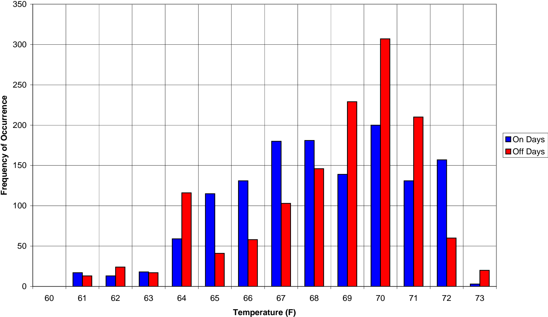
Atlantic City - Civil Court House Space Temperature Histogram (12/12/07 - 1/8/08)
