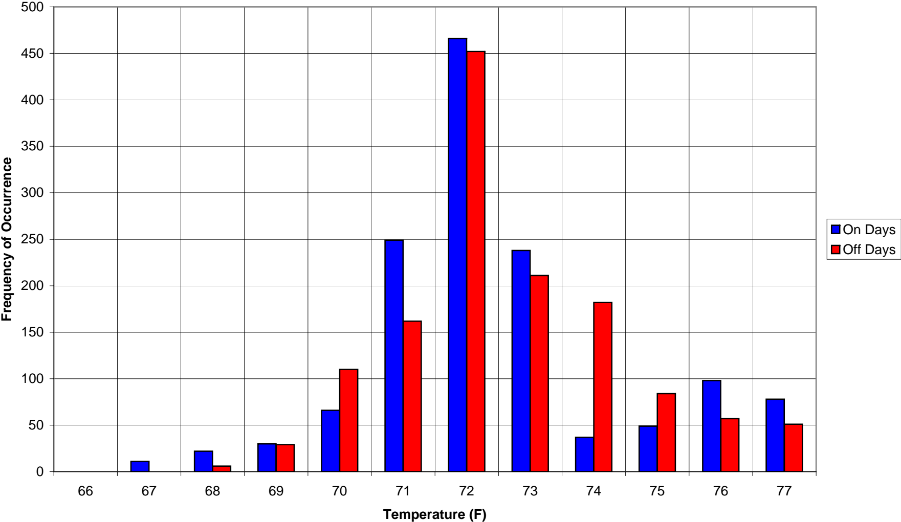
Atlantic City - County Office Building Space Temperature Histogram (12/12/07 - 1/8/08)
