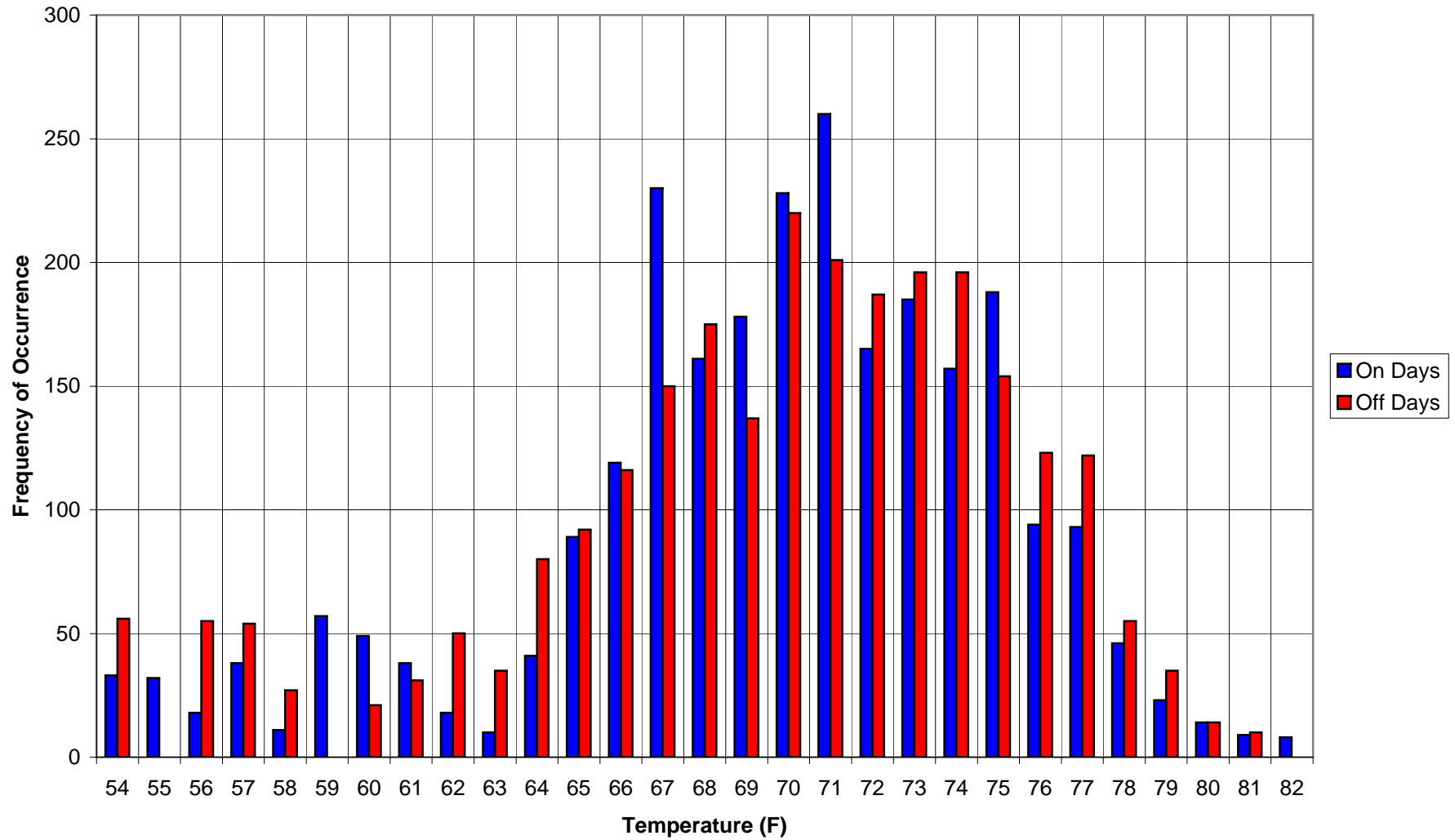
Middletown Village School Classroom "B" Temperature Histogram (03/07/07 - 4/29/07)
