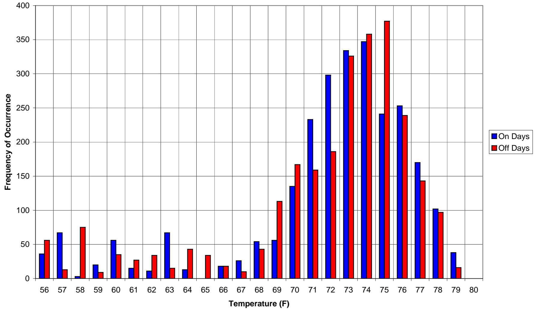
Middletown Village School Classroom "A" Temperature Histogram (03/07/07 - 4/29/07)
